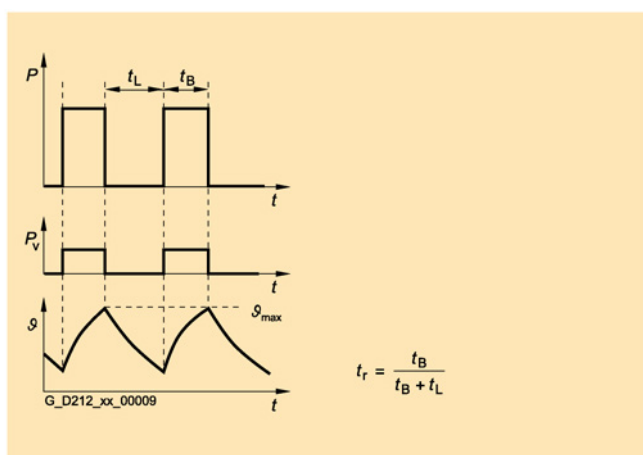
Image 4-4 S3 duty (intermittent operation without influencing starting)
