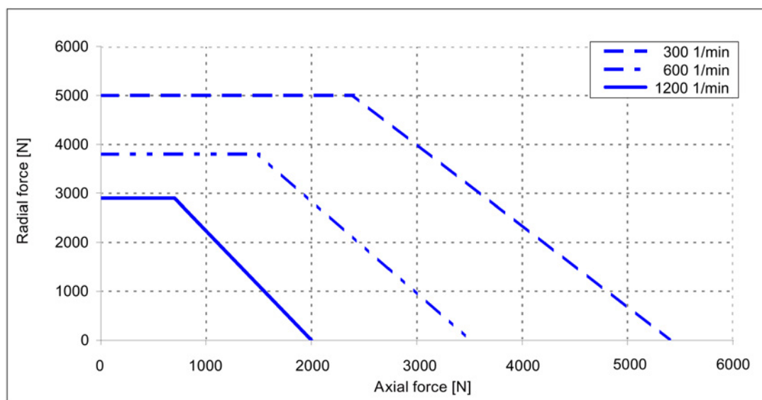
Image 3-17 Permissible axial force as a function of radial force for 1FW320□
