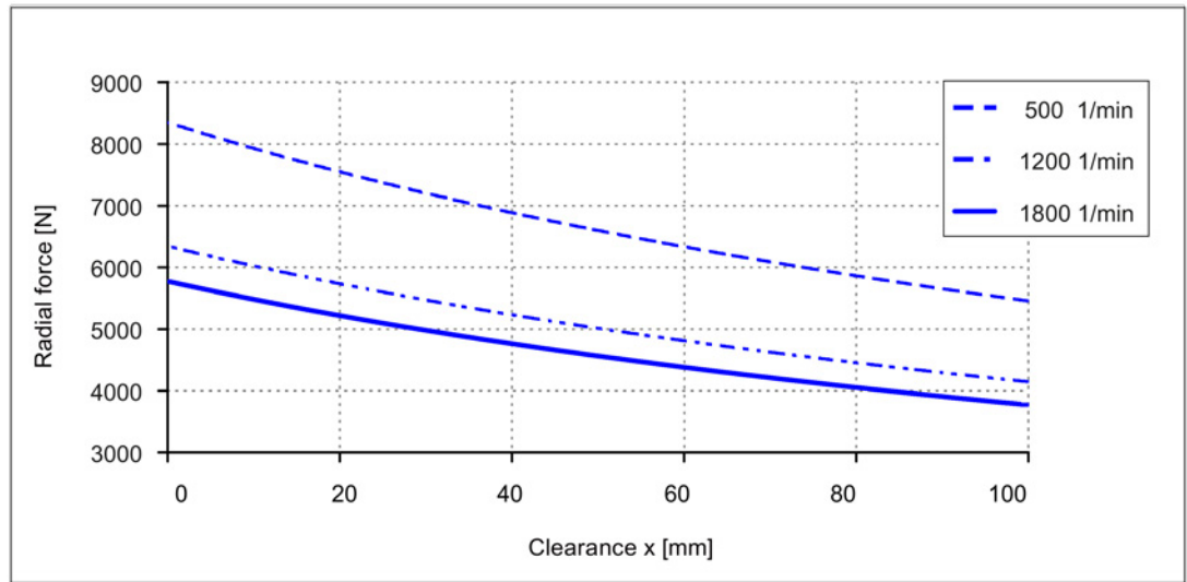
Image 3-24 Radial force diagram for 1FW320□, with nominal bearing change interval of 20000 h
