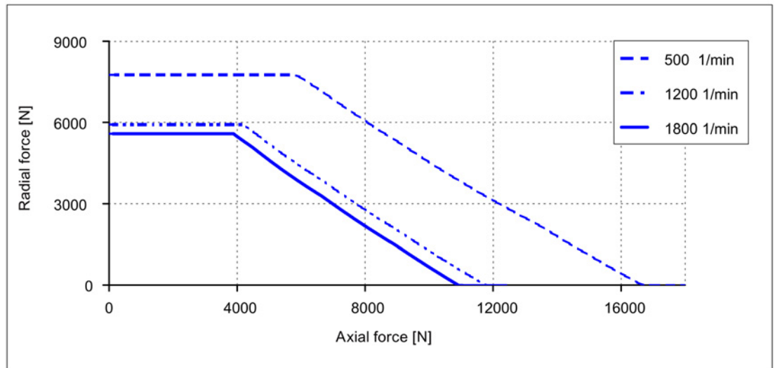
Image 3-33 Permissible axial force as a function of radial force for 1FW320□ (20000 h)
