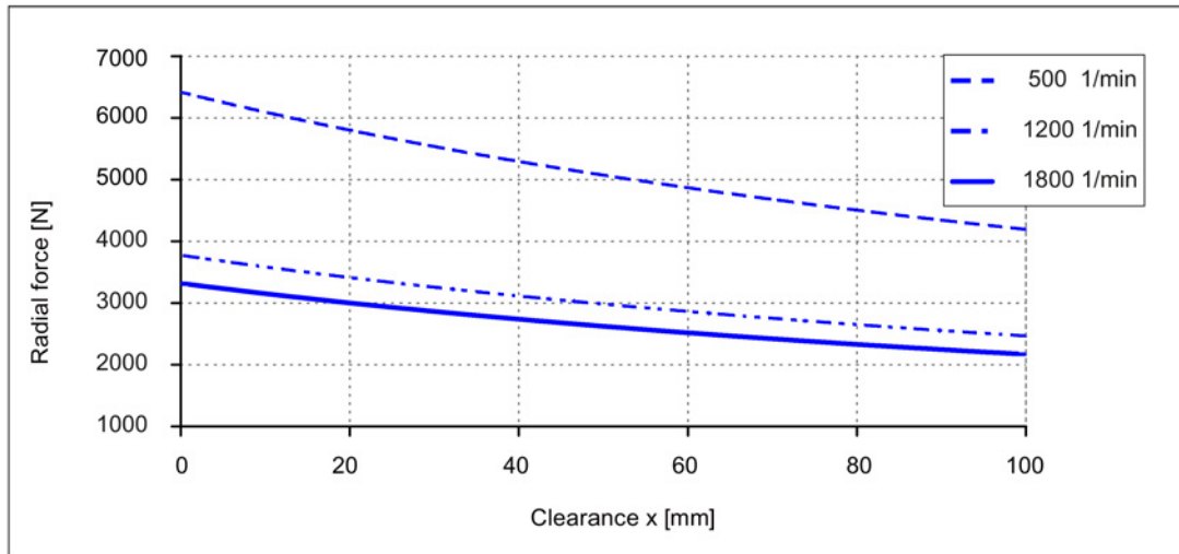
Image 3-26 Radial force diagram for 1FW320□, with nominal bearing change interval of 60000 h
