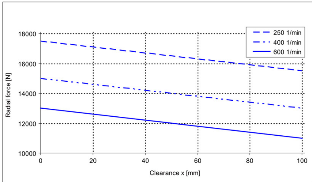
Image 3-18 Radial force diagram for 1FW328□, with nominal bearing change interval of 20000 h
