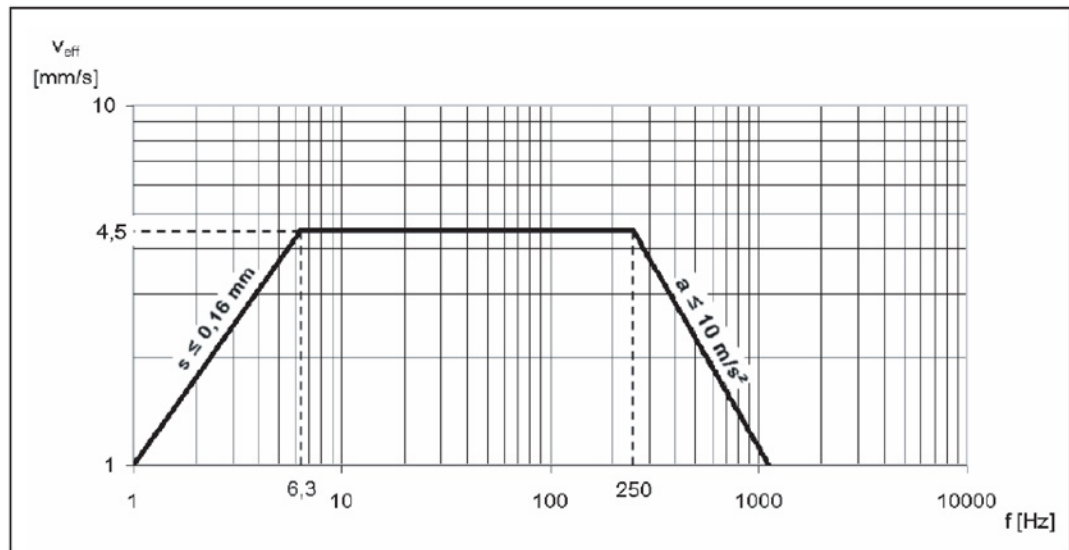
Image 6-27 Max. permissible vibration velocity, taking into account the vibration displacement and vibration acceleration
