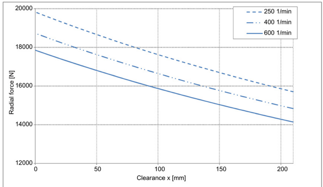
Image 3-36 Radial force diagram for 1FW328□, with nominal bearing change interval of 40000 h
