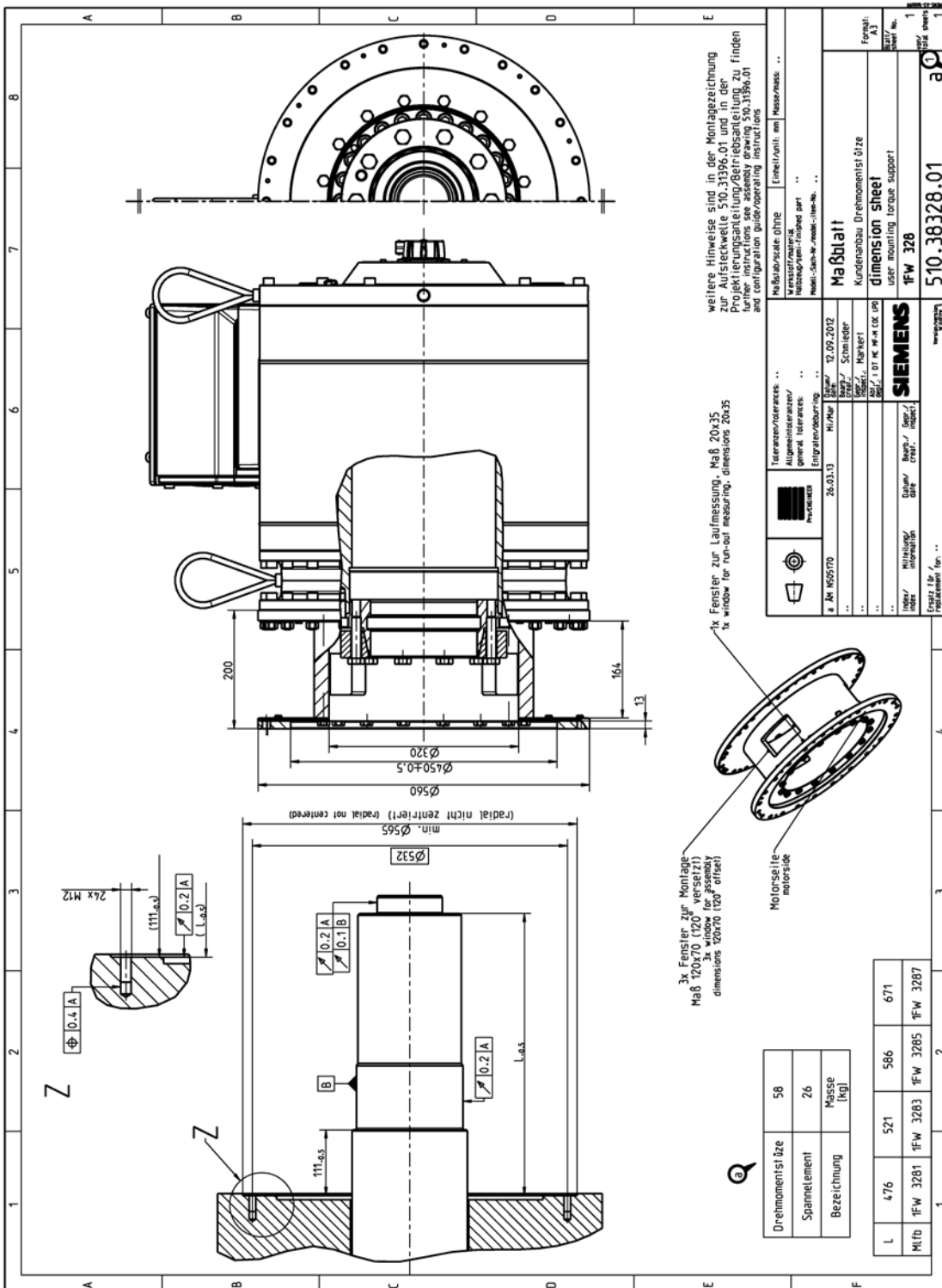
Image 6-13 1FW328 Siemens torque arm, dimension drawing 510.38328.01
