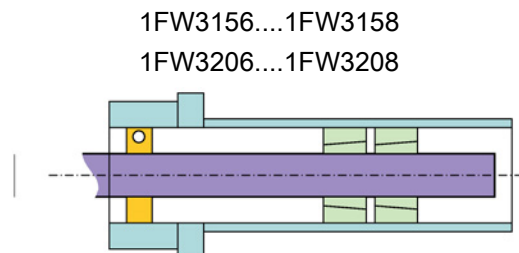
Two clamping sets are required to transmit the torque
