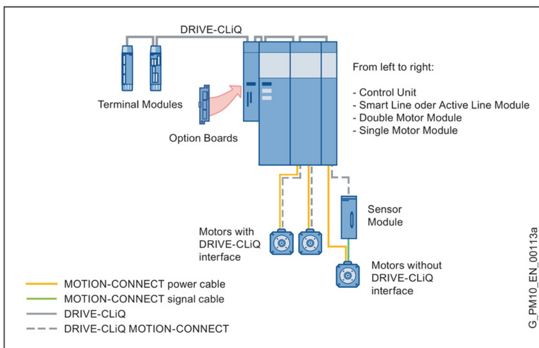
Image 7-1 SINAMICS S120 system overview
