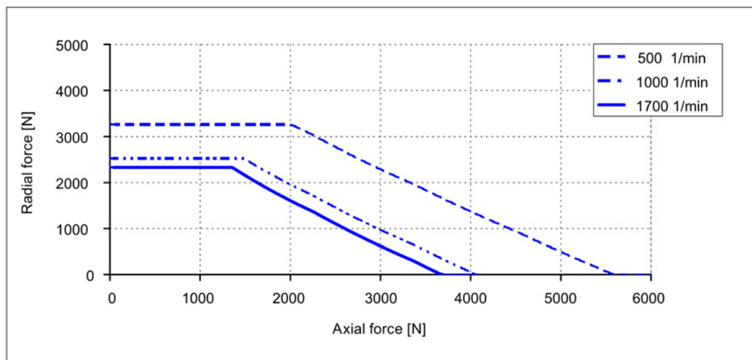
Image 3-31 Permissible axial force as a function of radial force for 1FW315□ (60000 h)
