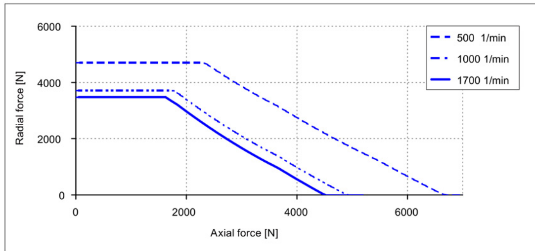
Image 3-23 Permissible axial force as a function of radial force for 1FW315□ (60000 h)
