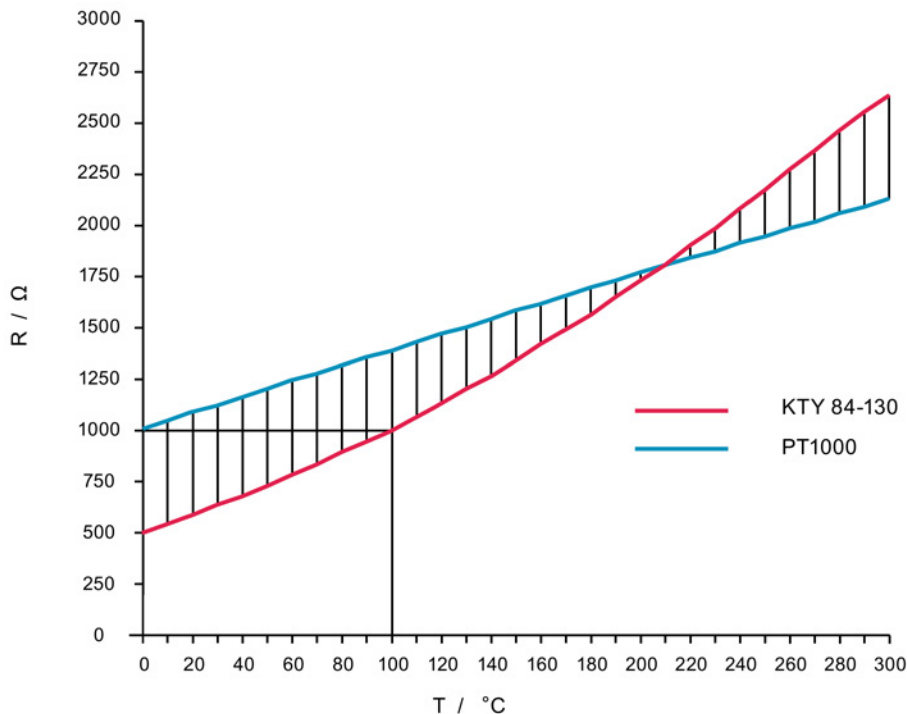
Image 3-1 Comparison of KTY 84-130 and Pt1000 temperature sensors
