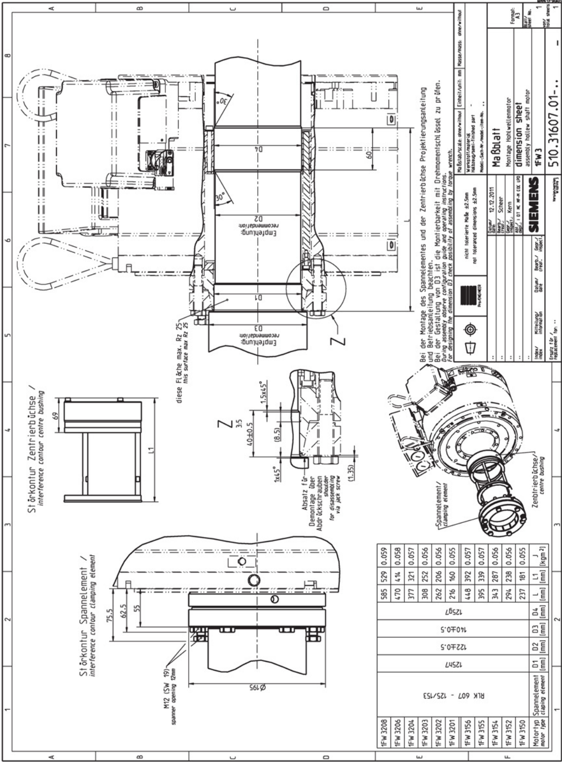
Image 6-19 Dimension drawing hollow shaft with clamping element
