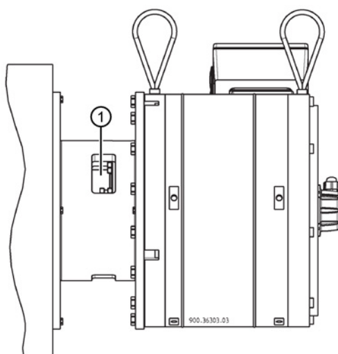
Image 6-8 Pre-mounting
