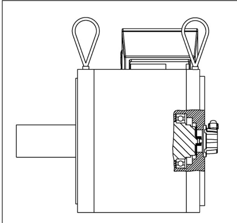
Image 3-6 Coaxial encoder mounting
