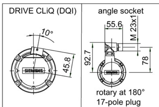
Image 10-13 Direct encoder mounting
