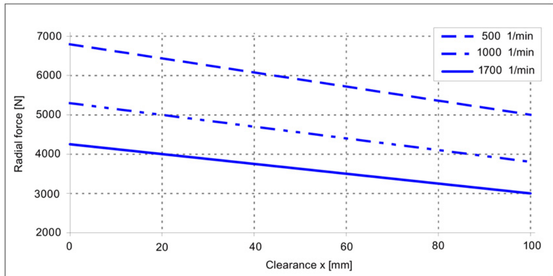
Image 3-14 Radial force diagram for 1FW315□, with nominal bearing change interval of 20000 h
