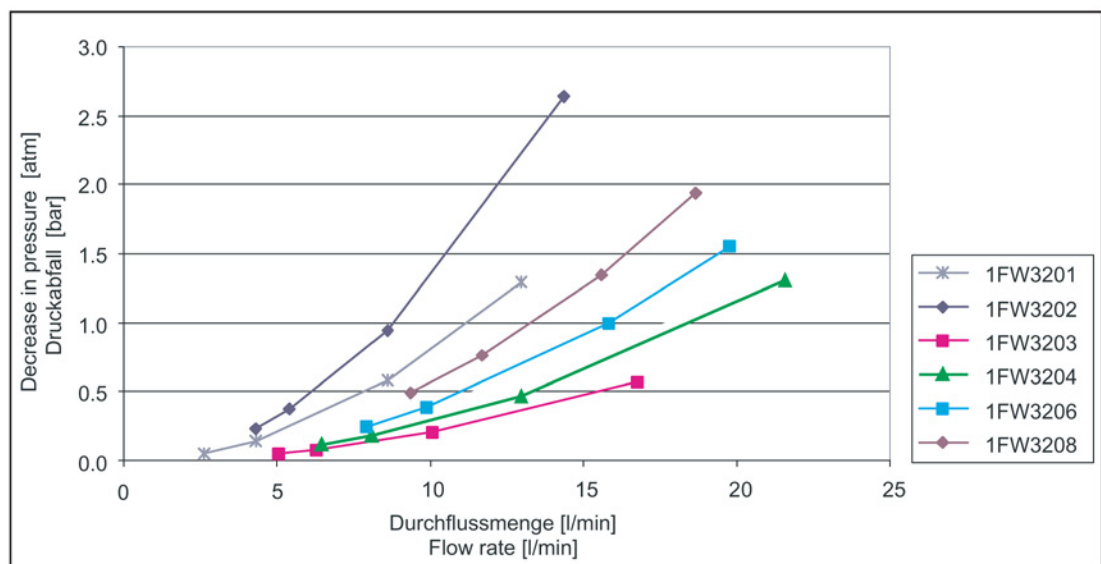
Image 3-9 Flow rate for SH 200
