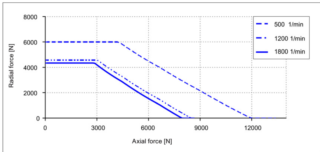
Image 3-35 Permissible axial force as a function of radial force for 1FW320□ (60000 h)
