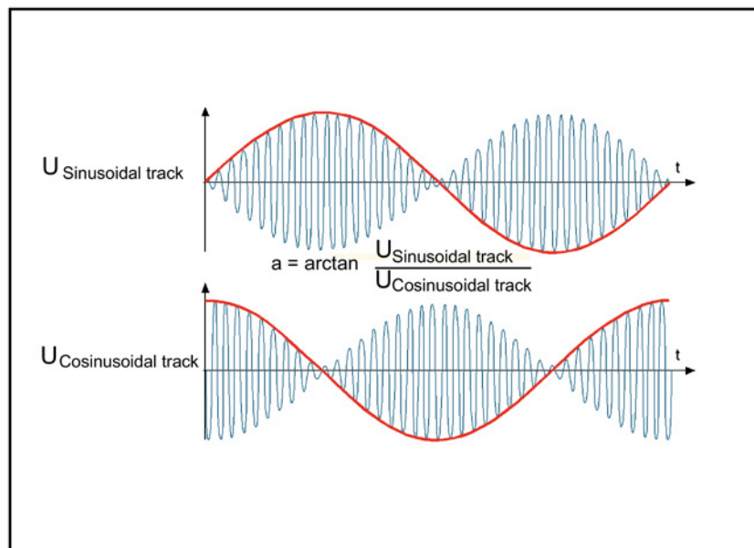
Image 3-4 Output signals, resolver
