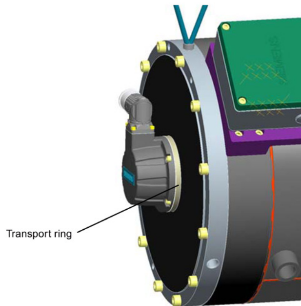
Image 6-25 Transport ring
