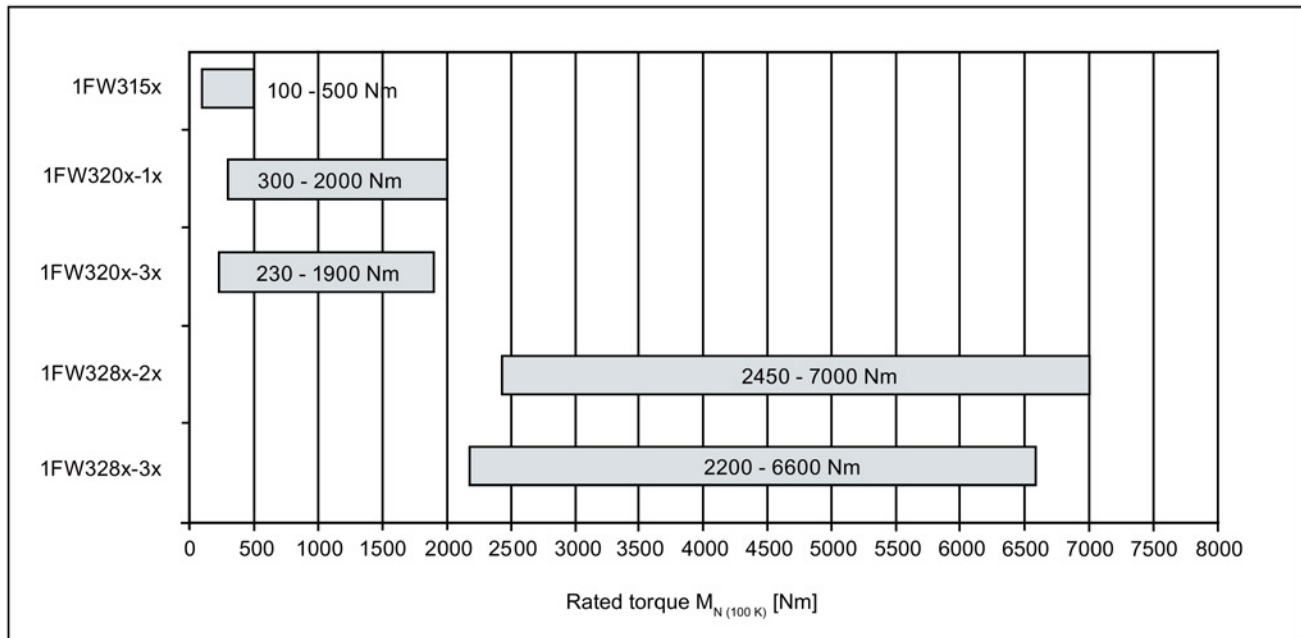
Image 2-2 Torque overview, 1FW3
