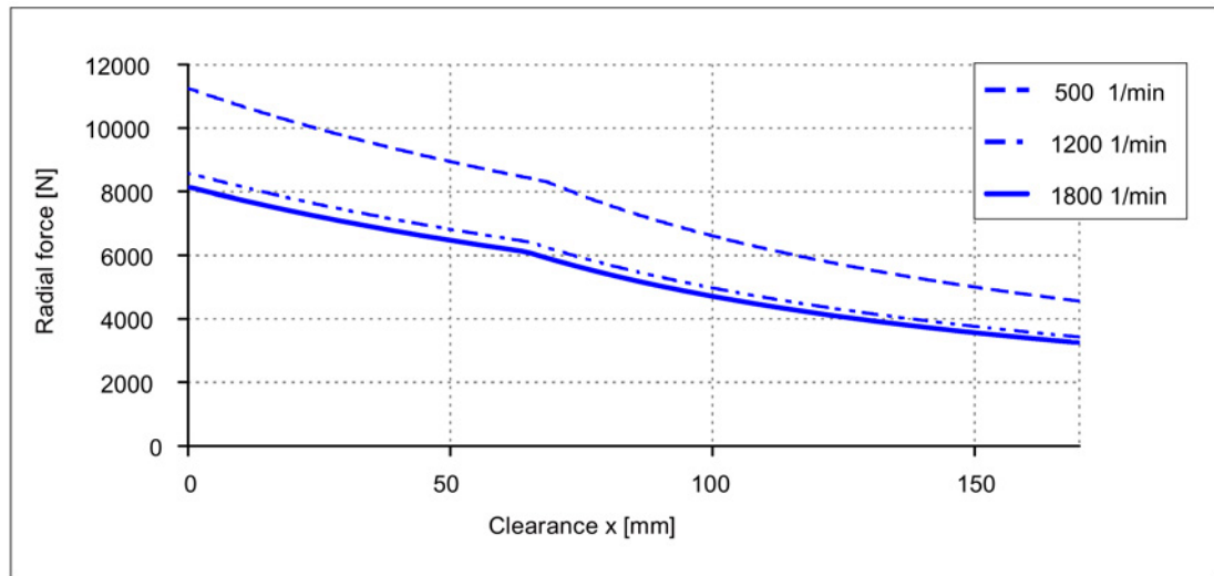
Image 3-34 Radial force diagram for 1FW320□, with nominal bearing change interval of 60000 h
