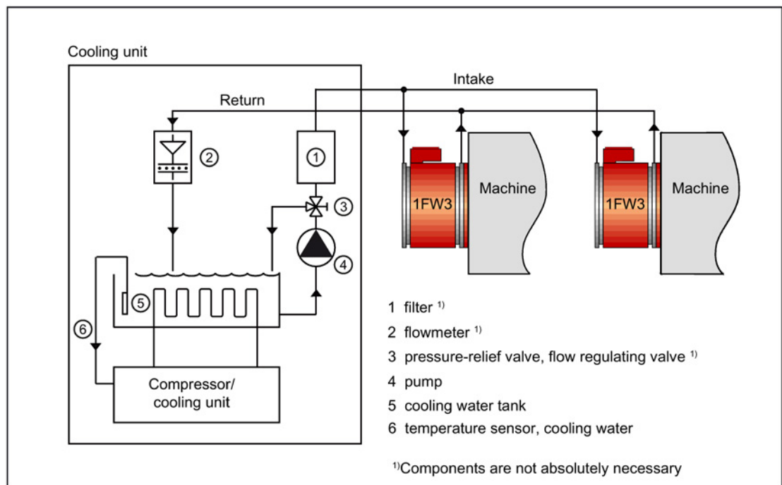
Image 3-7 Example of a semi-open cooling circuit
