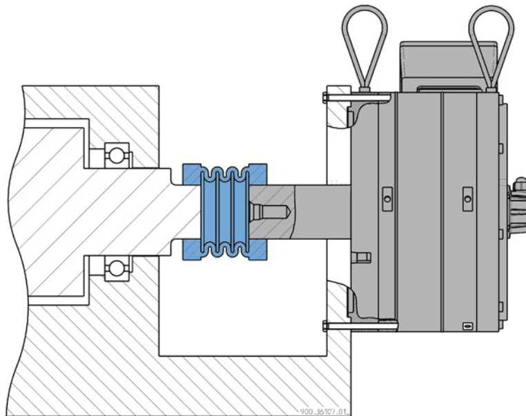
Image 6-22 Decoupling the machine shaft from the motor shaft using a coupling
