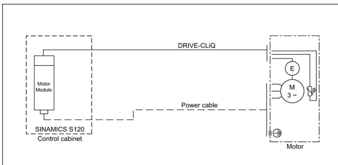
Image 7-5 Connecting encoders using the DRIVE-CLiQ interface
