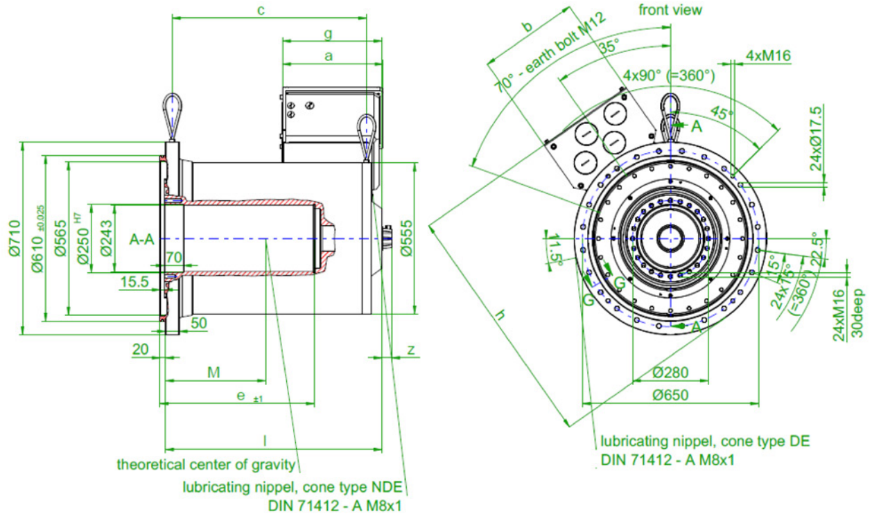
Image 10-12 SH 280, Heavy Duty
