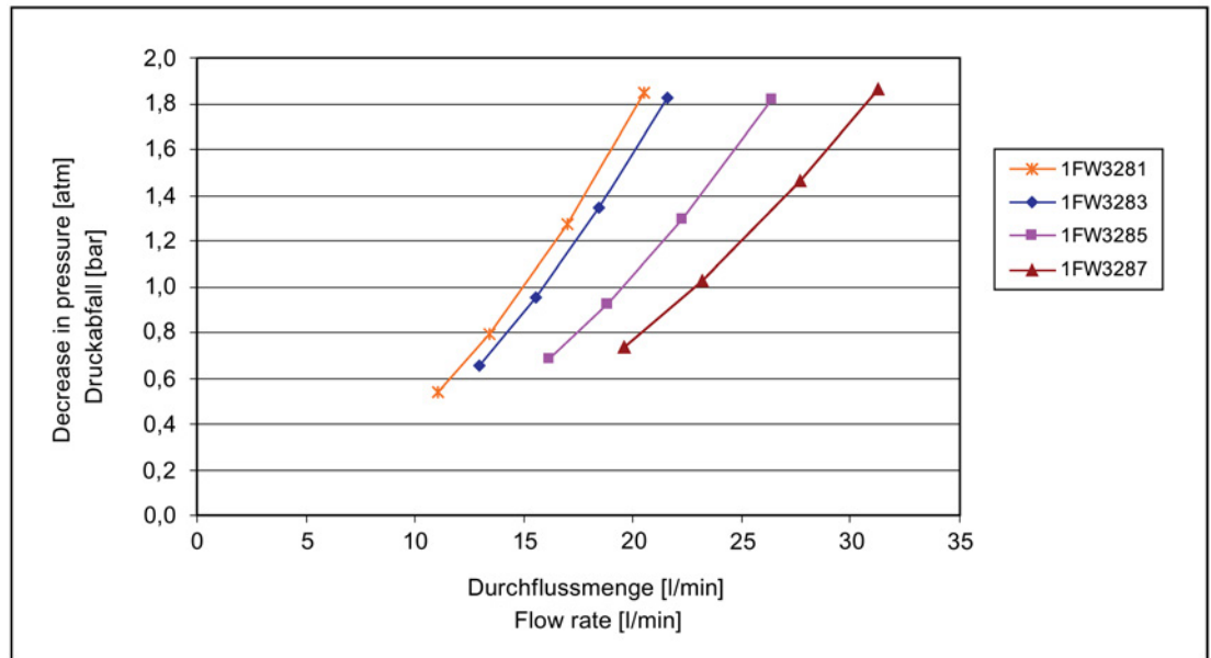
Image 3-10 Flow rate for SH 280
