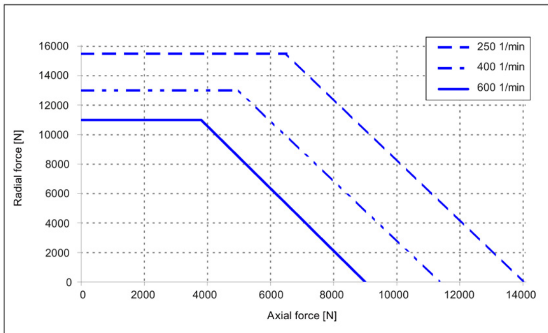
Image 3-19 Permissible axial force as a function of radial force for 1FW328□
