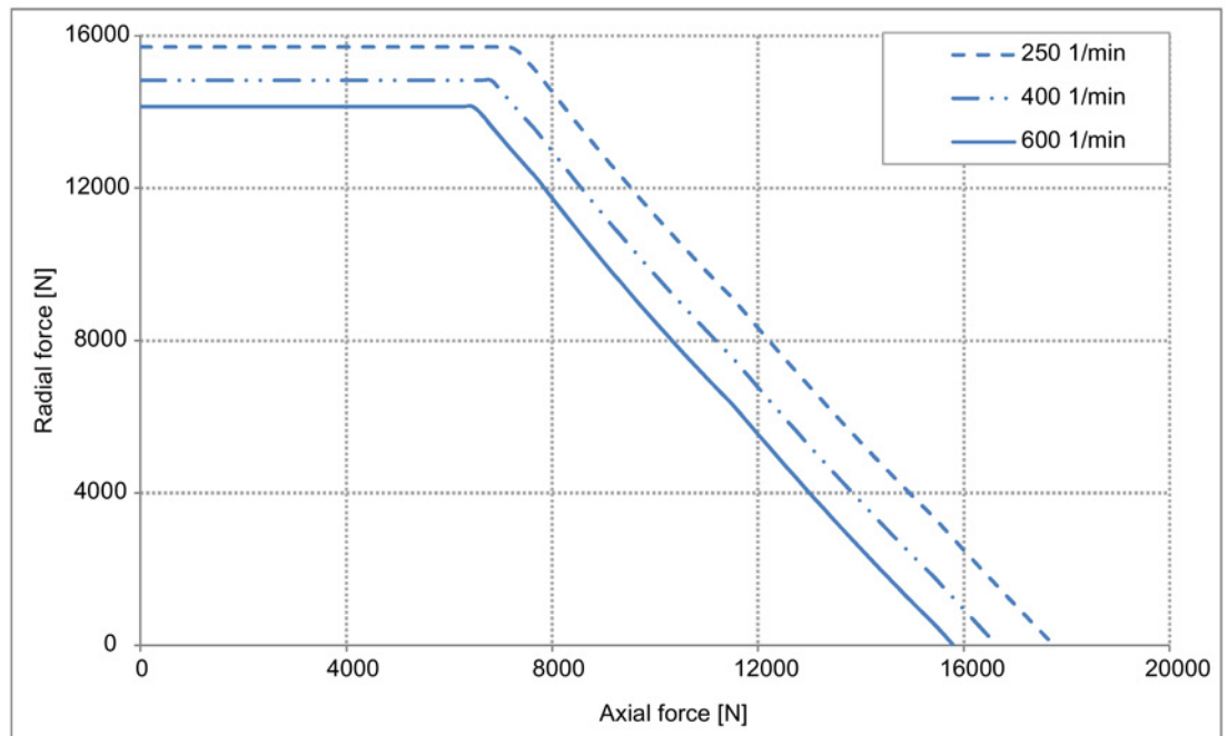
Image 3-37 Permissible axial force as a function of radial force for 1FW328□ (40000 h)
