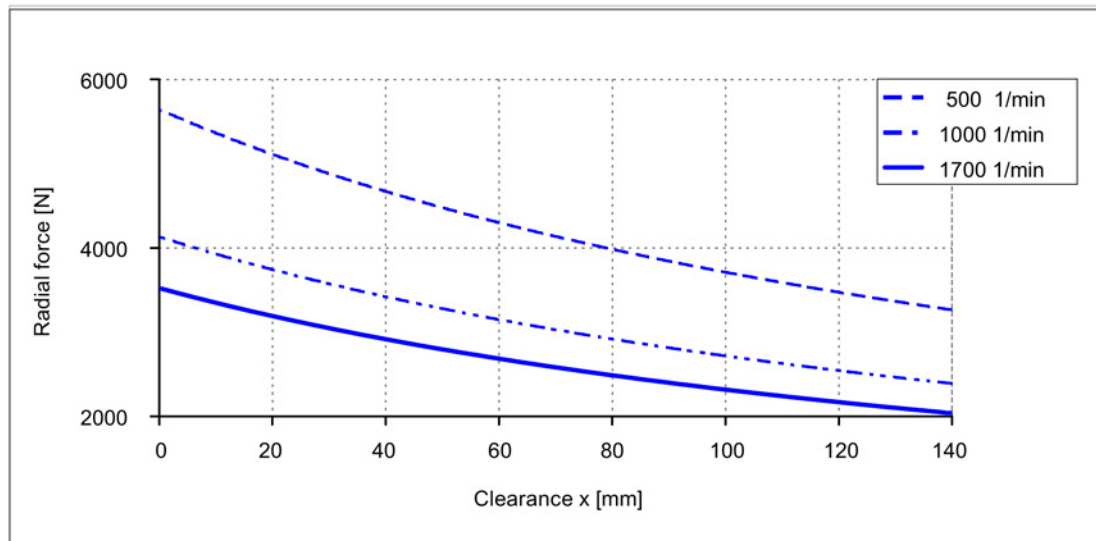
Image 3-30 Radial force diagram for 1FW315□, with nominal bearing change interval of 60000 h
