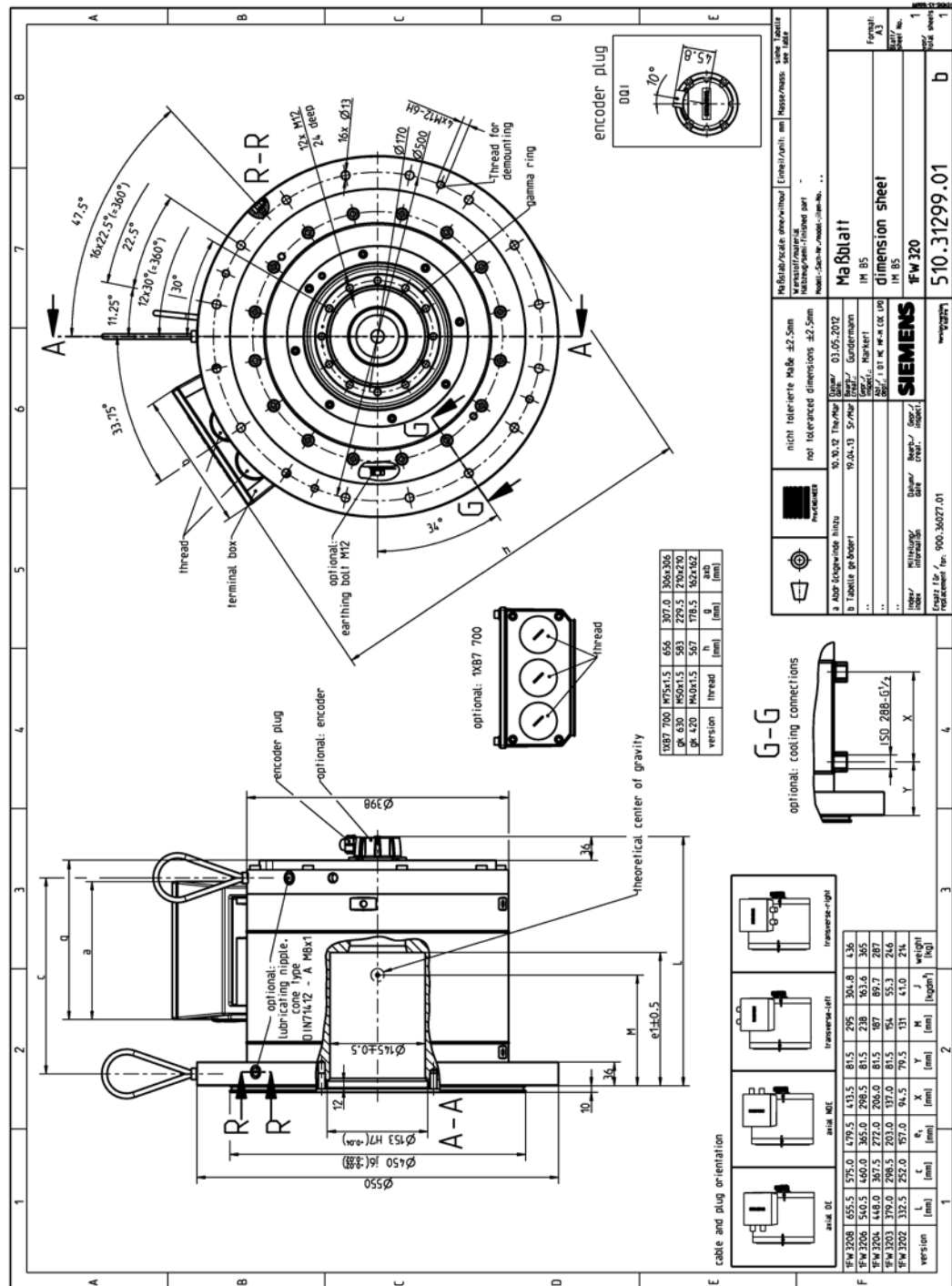
Image 6-28 1FW3 heavy duty SH 200
