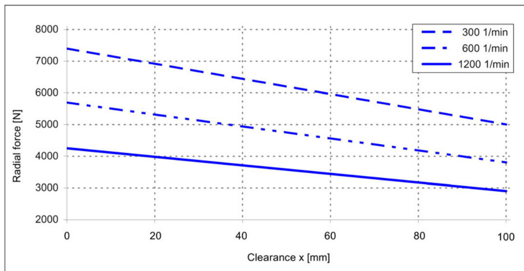
Image 3-16 Radial force diagram for 1FW320□, with nominal bearing change interval of 20000 h
