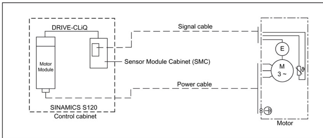
Image 7-6 Connecting encoders without DRIVE-CLiQ interface
