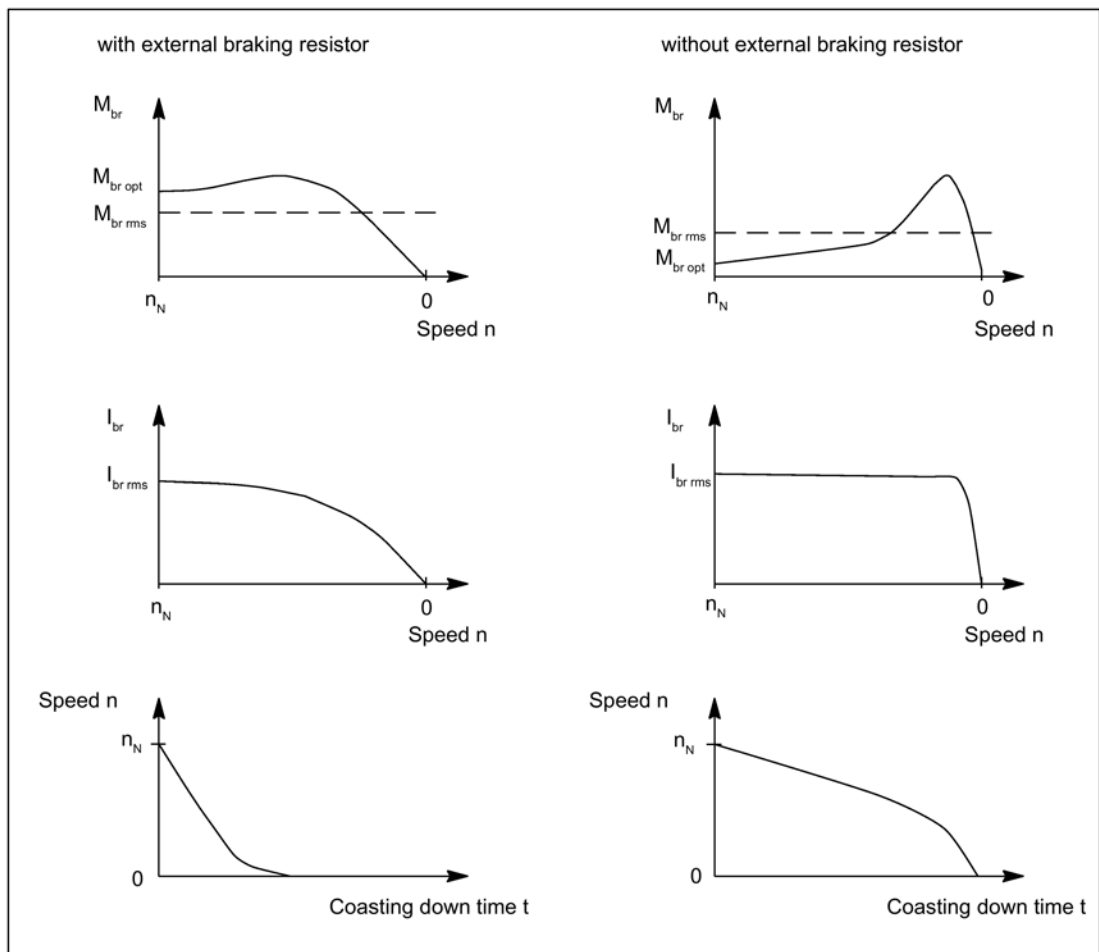
Image 3-12 Armature short-circuit braking
