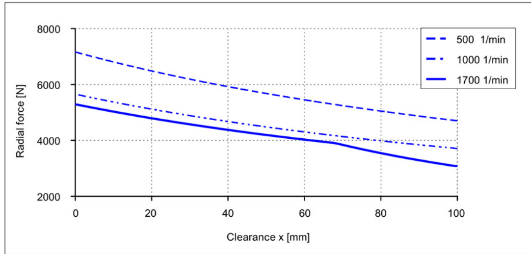
Image 3-22 Radial force diagram for 1FW315□, with nominal bearing change interval of 60000 h
