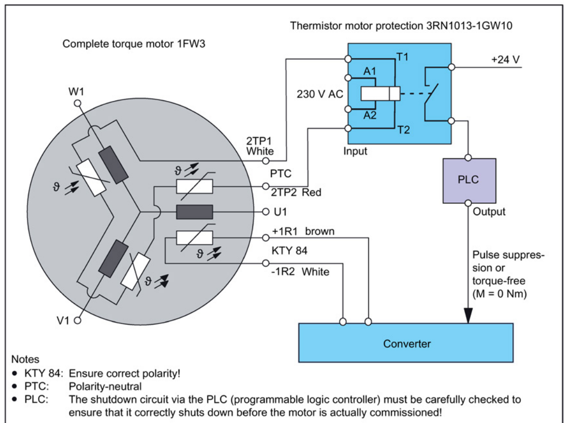
Image 3-2 Temperature monitoring connection
