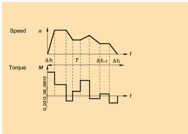
Image 4-6 Example of a load duty cycle
