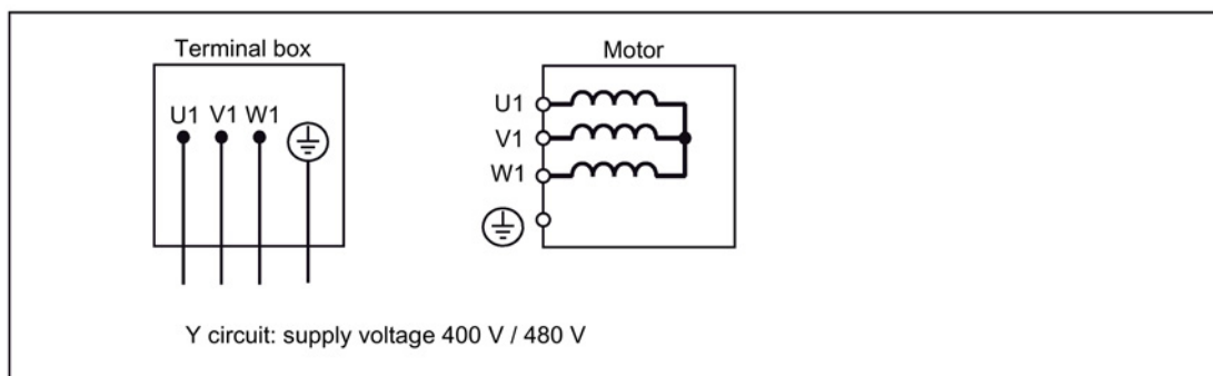
Image 7-3 Circuit diagram
