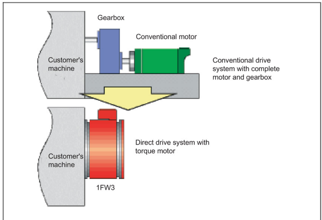
Image 6-1 Comparison between conventional and direct drive systems
