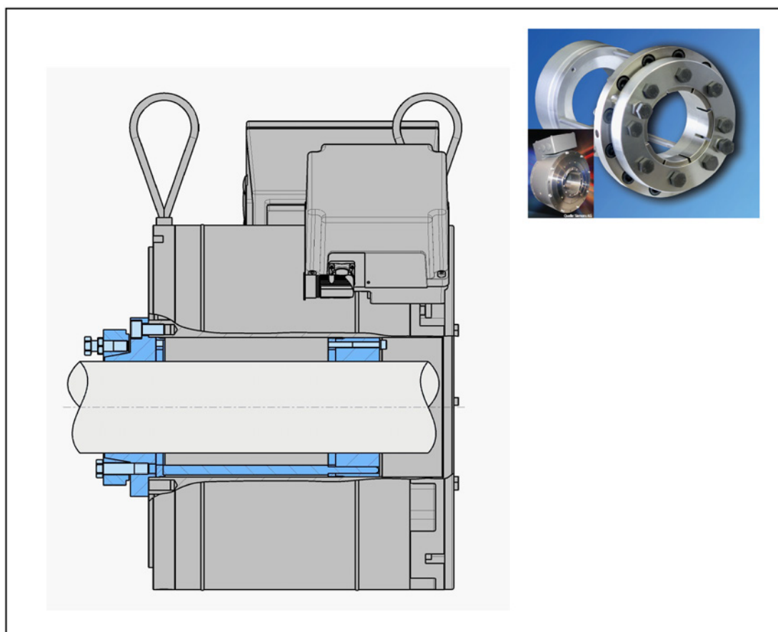
Image 6-18 Outer clamping system
