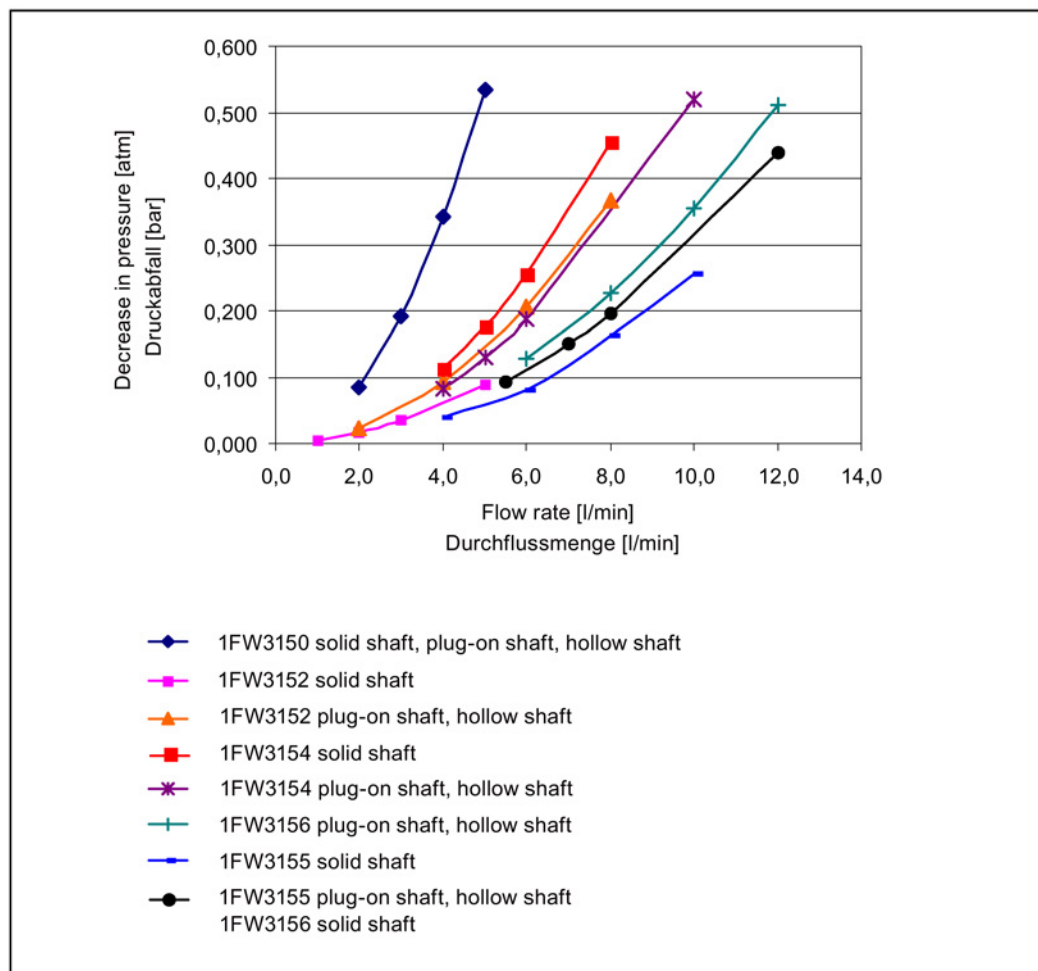
Image 3-8 Flow rate for SH 150
