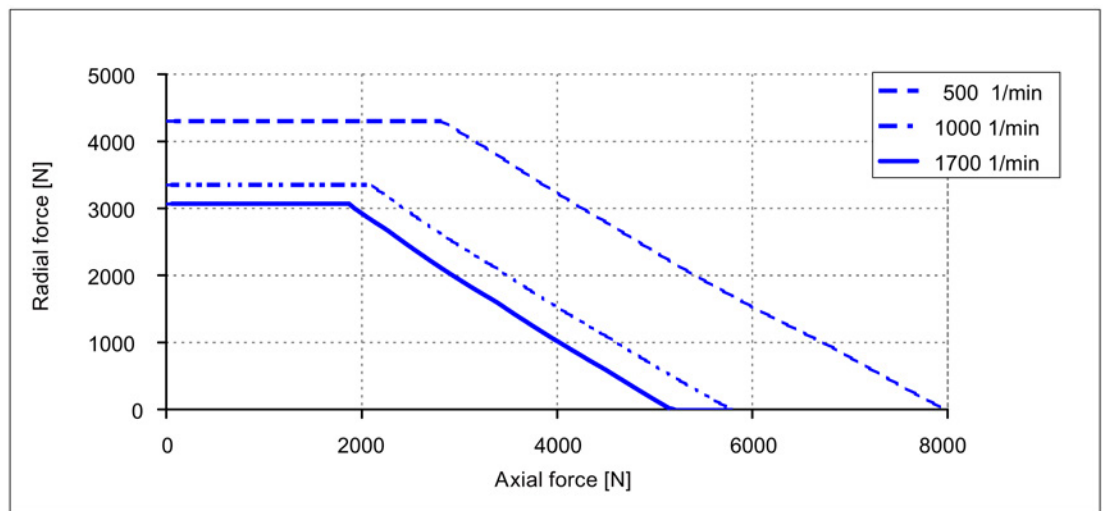
Image 3-29 Permissible axial force as a function of radial force for 1FW315□ (20000 h)
