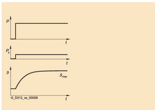
Image 4-3 S1 duty (continuous operation)
