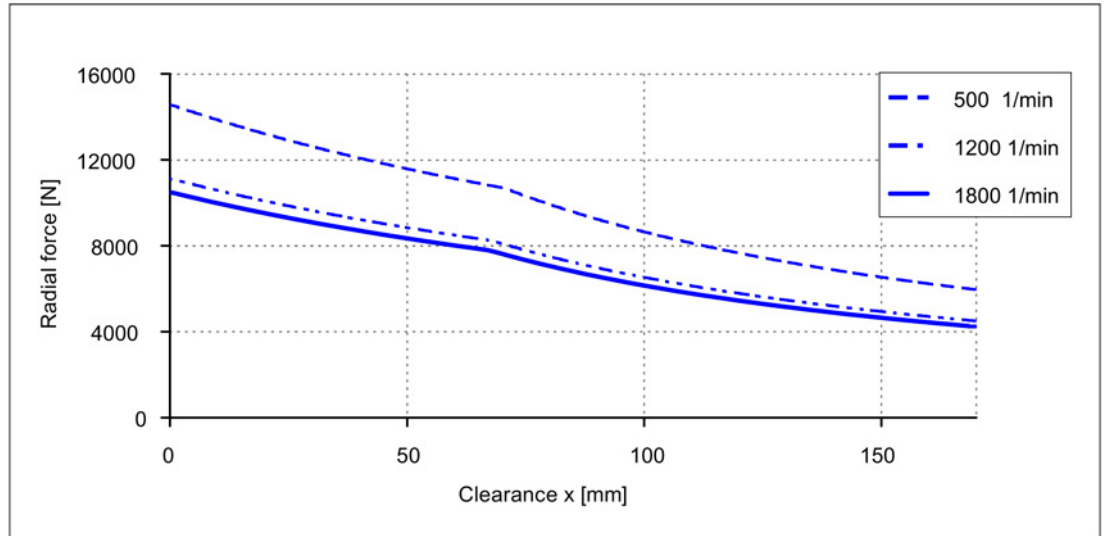
Image 3-32 Radial force diagram for 1FW320□, with nominal bearing change interval of 20000 h
