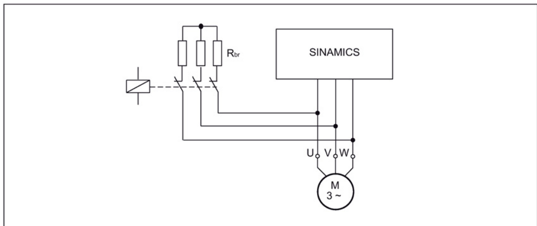
Image 3-11 Circuit (schematic) with brake resistors
