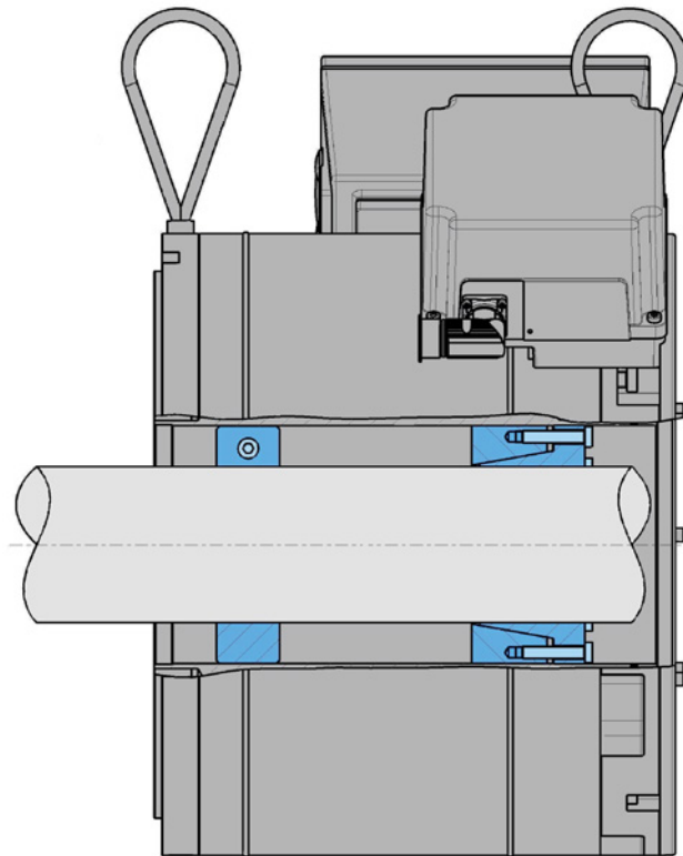
Image 6-20 Inner clamping system
