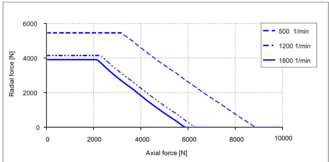
Image 3-25 Permissible axial force as a function of radial force for 1FW320□ (20000 h)
