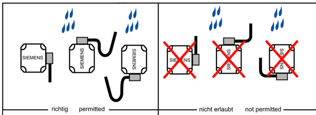
Image 7-7 Principle of cable routing in a wet/moist environment
