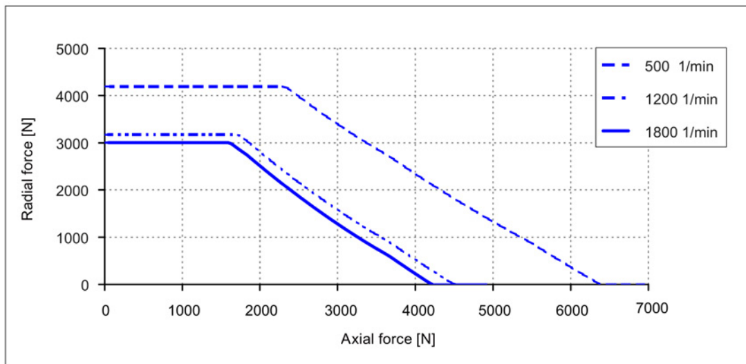
Image 3-27 Permissible axial force as a function of radial force for 1FW320□ (60000 h)
