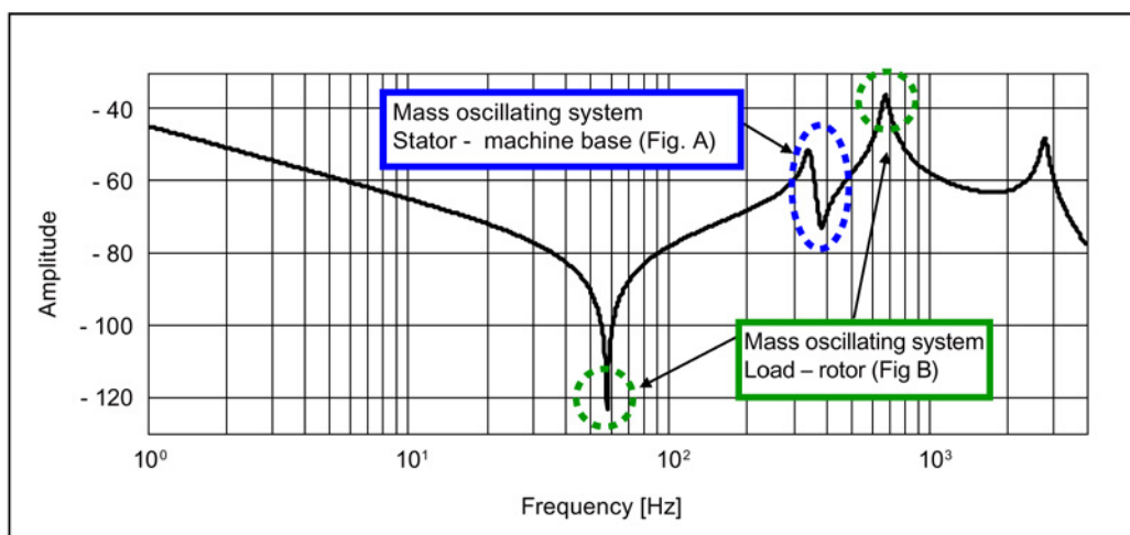
Image 6-5 Speed control loop – influence of the Siemens torque arm
