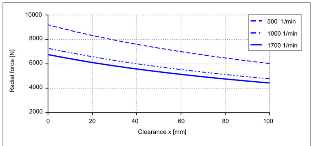
Image 3-20 Radial force diagram for 1FW315□, with nominal bearing change interval of 20000 h
