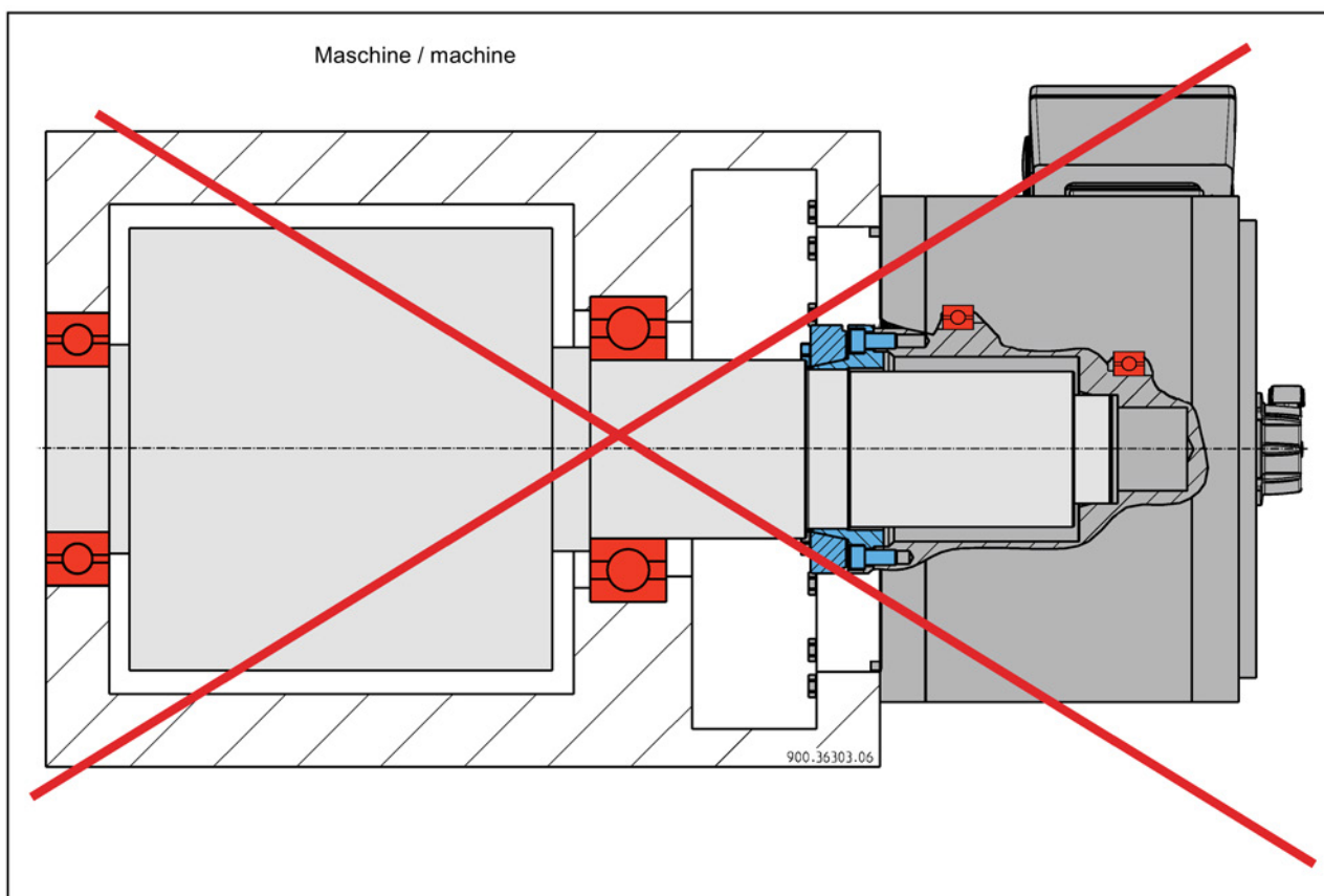
Image 6-2 Over-determined bearings of a shaft (to be avoided)
