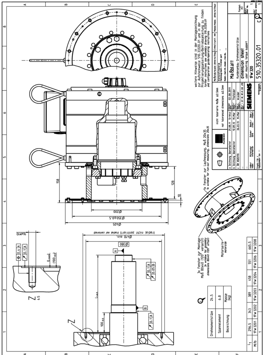
Image 6-12 1FW320 Siemens torque arm, dimension drawing 510.35320.01
