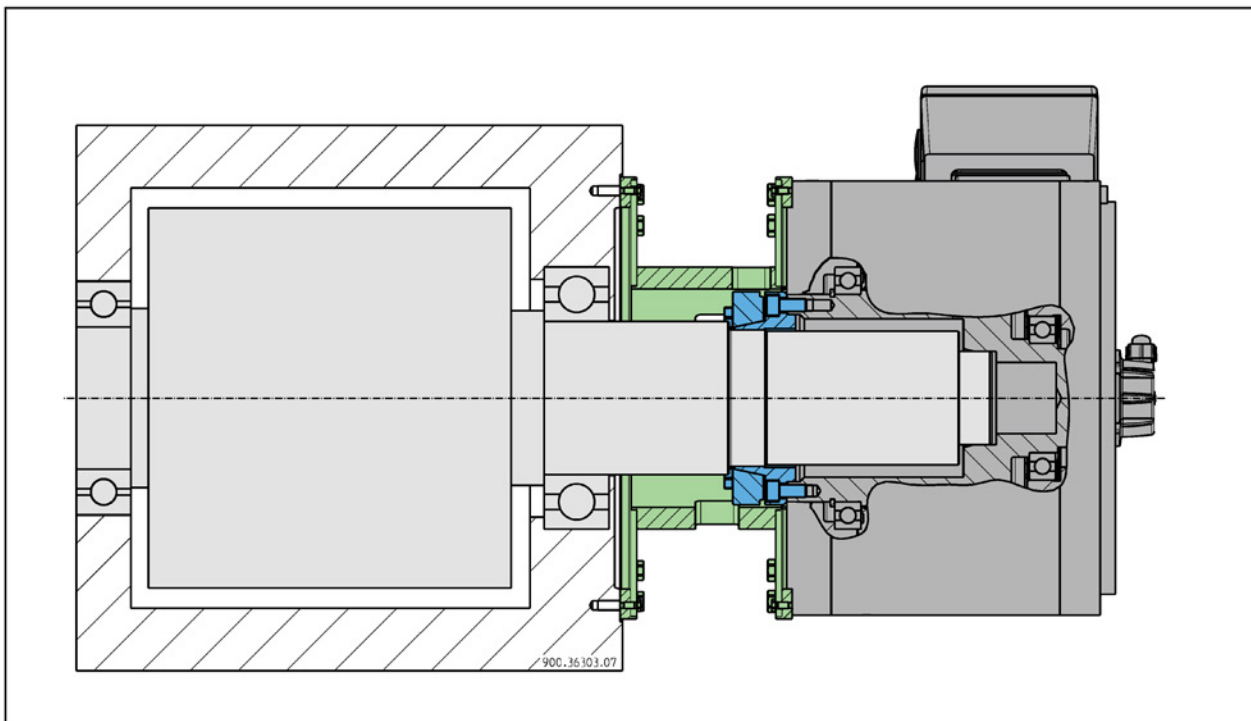
Image 6-4 Schematic representation of the Siemens torque arm
