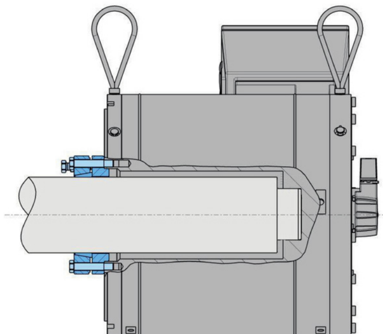
Image 6-14 Plug-on shaft clamping element
