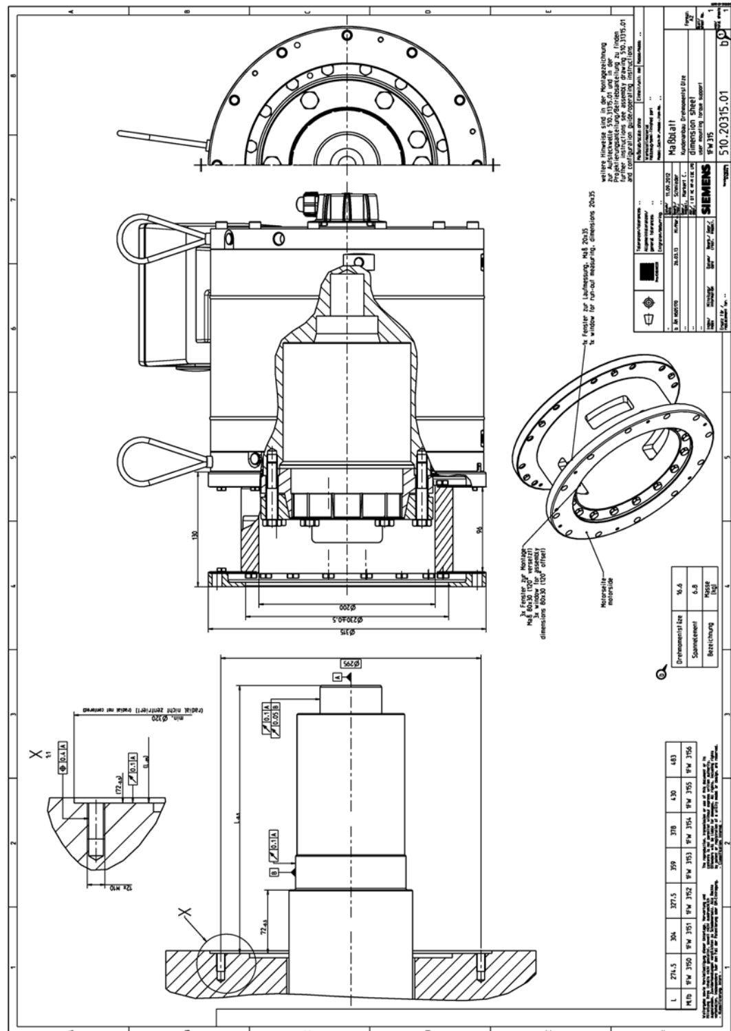
Image 6-11 1FW3150 Siemens torque arm, dimension drawing 510.20315.01
