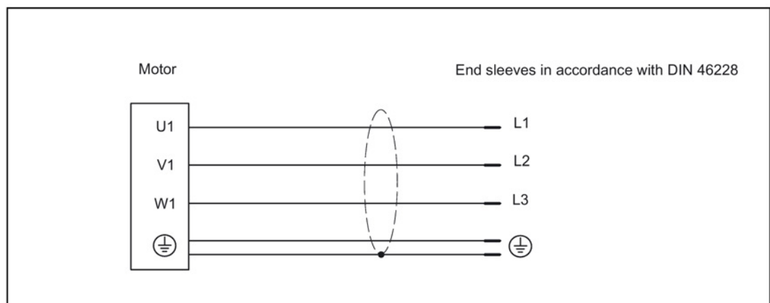
Image 7-2 Power cable
