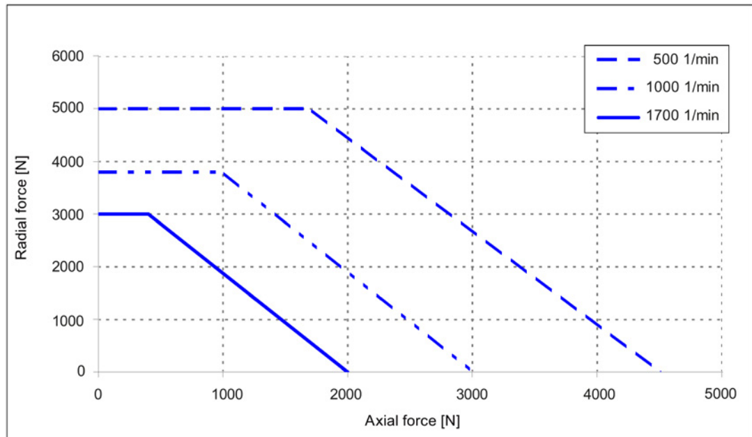
Image 3-15 Permissible axial force as a function of radial force for 1FW315□
