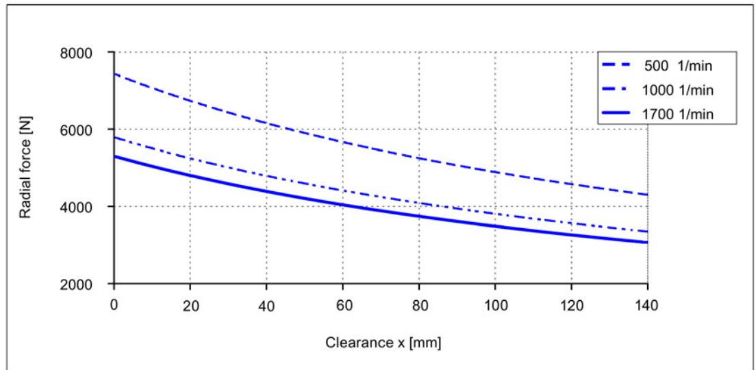
Image 3-28 Radial force diagram for 1FW315□, with nominal bearing change interval of 20000 h
