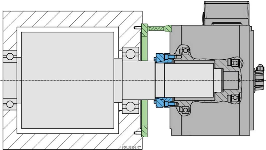
Image 6-3 Decoupling the stator from the machine base using a torque arm (schematic representation)
