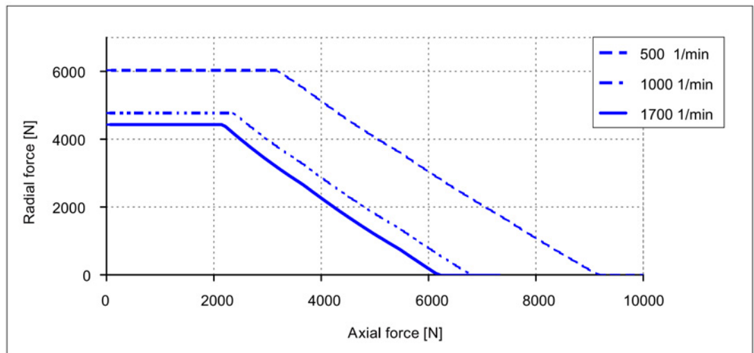
Image 3-21 Permissible axial force as a function of radial force for 1FW315□ (20000 h)
